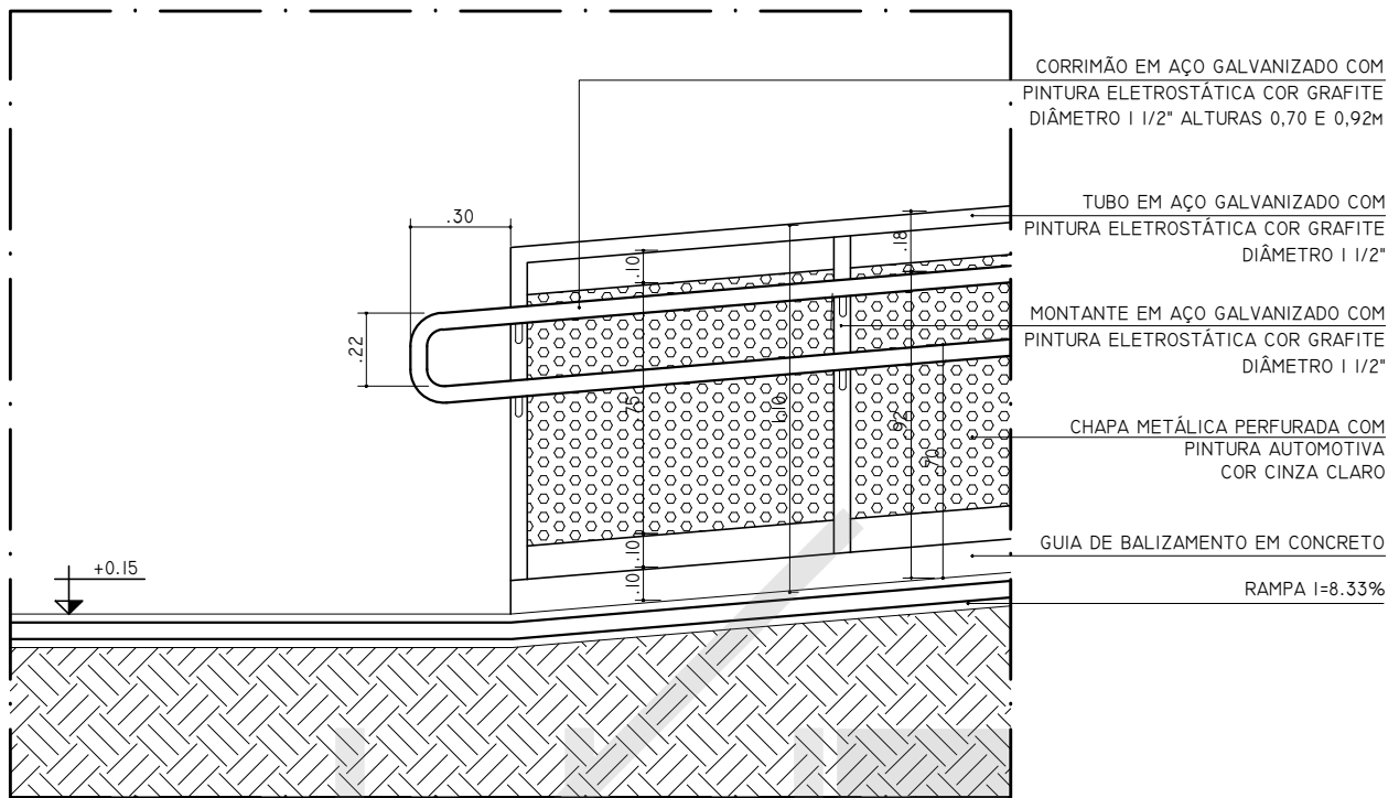
VISTA LATERAL RAMPAS (LATERAL)
